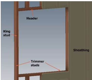
Sheathed Wall
